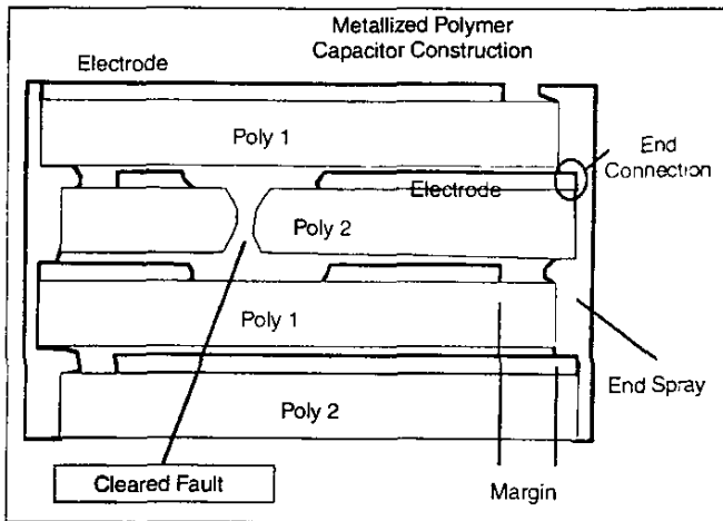
Fig. 2 Typical metallized polypropylene capacitor winding cross-section after a "clearing" event has taken place. The capacitor's electrode is deposited on the dielectric prior to winding the capacitor and the current-carrying electrodes are explicitly made extremely thin in order to enhance the clearing process both locally and throughout the capacitor.
