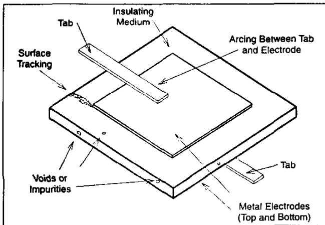
Fig. 1 Illustrates schematically a number of the more important technical design factors that influence the capacitor designer's choice of geometry, connections, and materials
