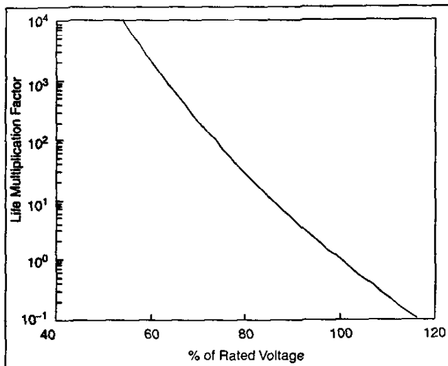
Fig. 4 Life multiplication factor as a percent of rated dc voltage
